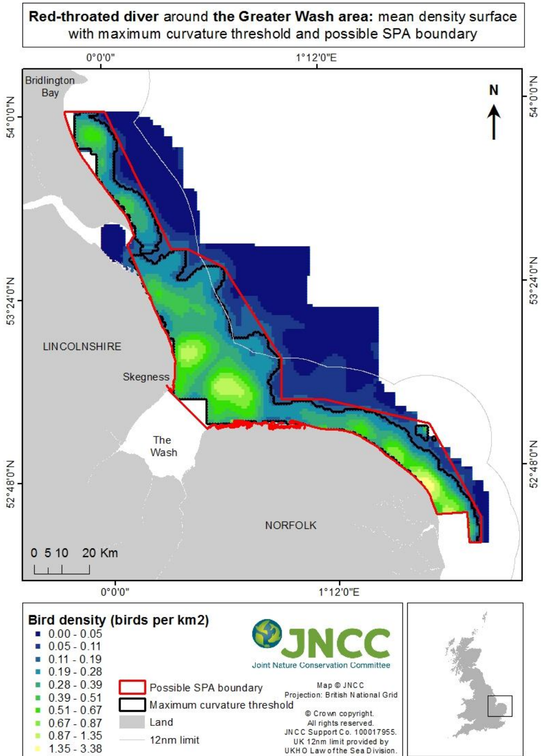
Figure A1. Estimated mean density surface for red-throated diver with the threshold densities delineated, as identified by maximum curvature (0.1665 birds per km 2 ) and the composite possible SPA boundary.
